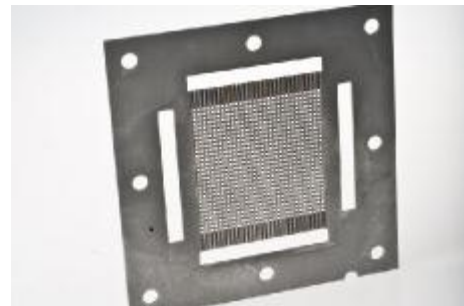
Fuel Cell ( Sheet size ; 90x90mm)
